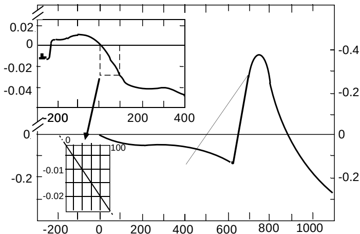
Figure 1 The temperature difference (t_{90} - t_{68})/^{\circ}\text{C} in the range between the triple point of equilibrium hydrogen (-259.3467^{\circ}\text{C}) and the freezing point of gold (1064.18^{\circ}\text{C}) [83.85]
