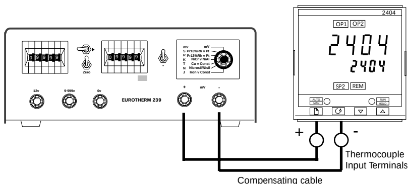
Figure 2 Type 239 Millivolt source
