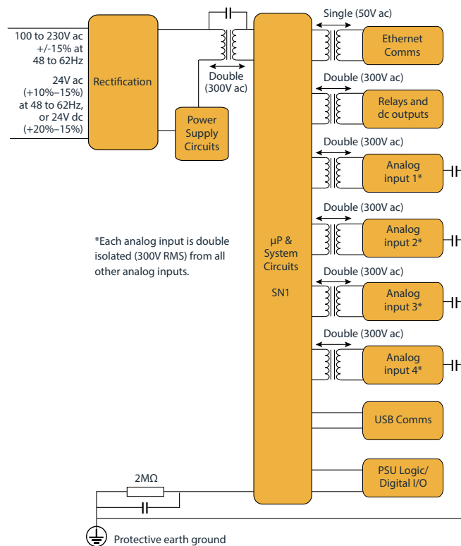
Isolation details
