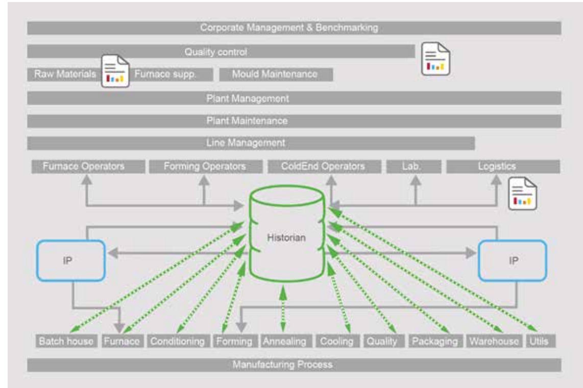
Collecting digital, analogue and 3rd party format plant data in a single historian server simplifies analysis and reporting at every level
